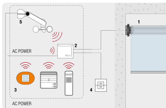
1. TUBULAR MOTOR 2. MINDY TT4 SERIES CONTROL UNIT 3. TRANSMITTER 4. "UP/DOWN" BUTTON CONNECTED TO THE MINDY TT4 SERIES CONTROL UNIT 5. NEMO SERIES RADIO-CONTROLLED ANEMOMETER
