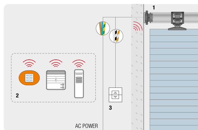
1. TUBULAR MOTOR 2. TRANSMITTER 3. "UP/DOWN" BUTTON CONNECTED TO THE TTBUS* OR PUSHBUTTON WITH ERA PLUS MH AND ERA PLUS LH
