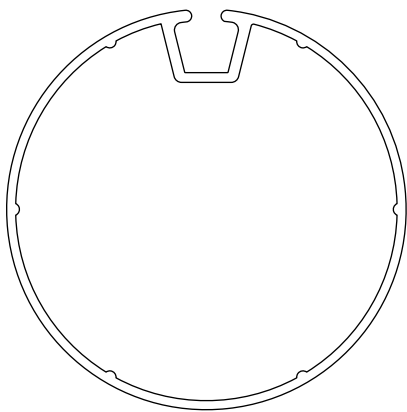
503.15300 Notch 53x1.5 wheel + crown
