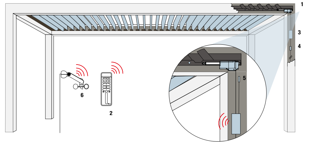
1. Motor 2. Transmitter 3. Control unit 4. Power Supply module 5. Temperature Sensor 6. Climatic sensor
