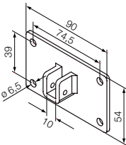
525.10074 max 30 Nm 90x54 flange with saddle bracket for 10 mm pin.
