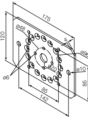
525.10089 175x120 support for sides
